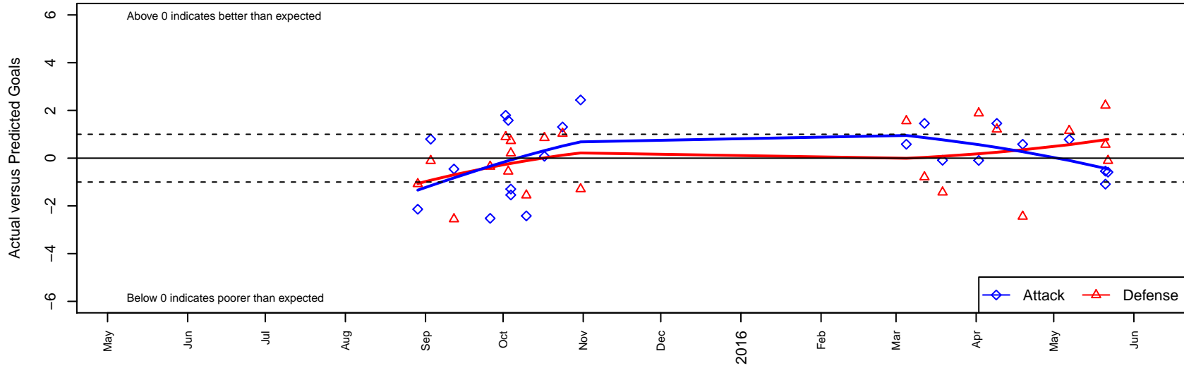
Idaho Inferno B04 Dots are actual minus expected GF (blue circles) and GA (red triangles). Blue line is smoothed change in attack strength. Red is smoothed change in defense strength.
